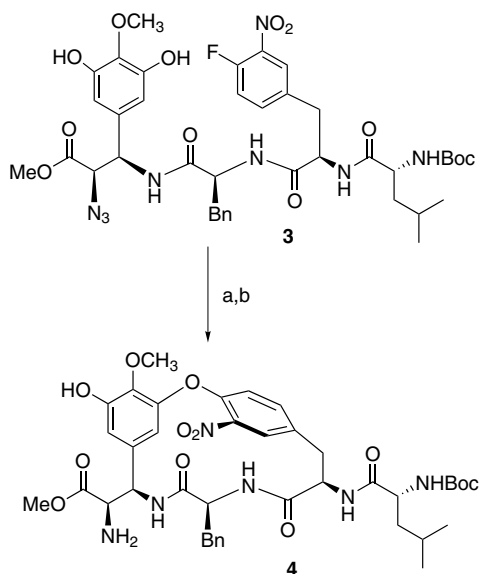
Scheme 1. (a) Ph_3P , THF- H_2O ; (b) CsF , DMSO, 0.01 M, room temperature.
