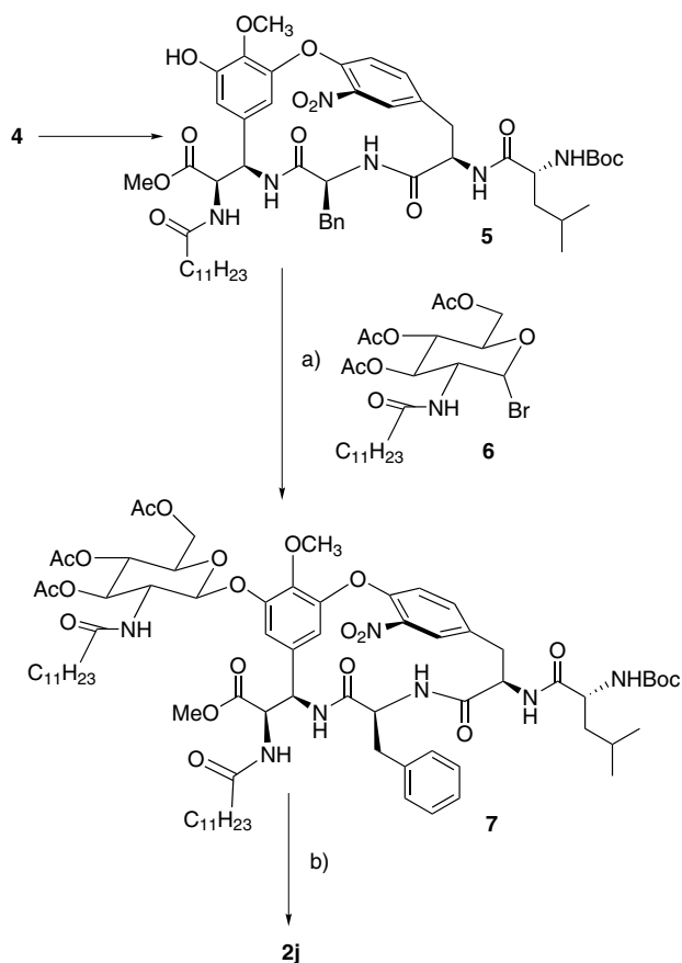
Scheme 2. (a) 10% \text{Na}_2\text{CO}_3 , ^t\text{Bu}_4\text{NHSO}_4 , \text{CH}_2\text{Cl}_2\text{--H}_2\text{O} , 75%; (b) \text{LiOH} , \text{THF--H}_2\text{O} , then 10% conc \text{HCl} in \text{CH}_3\text{CN} , 85%.
