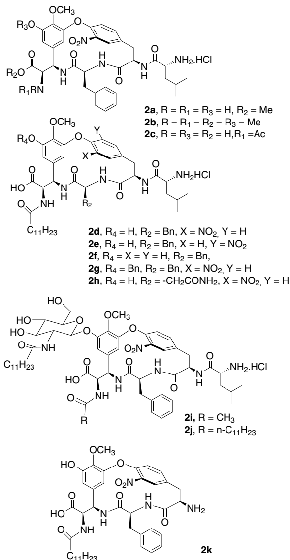
Figure 3. Structure of macrocycles.
