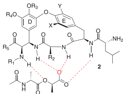
Figure 2. Generic structure of compound 2 and expected interaction with D-Ala-D-Lac.
