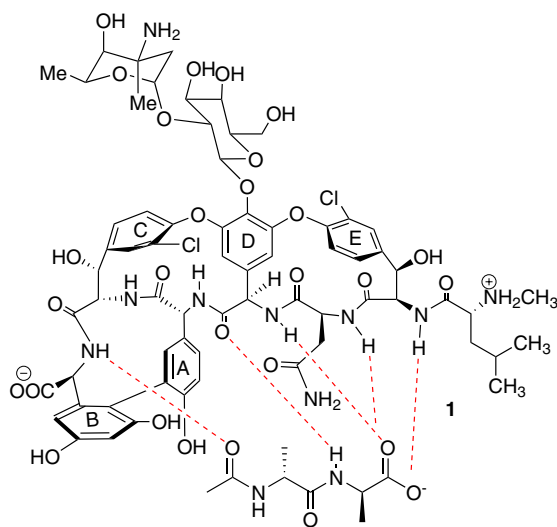
Figure 1. Vancomycin (1) and D-Ala-D-Ala complex.
